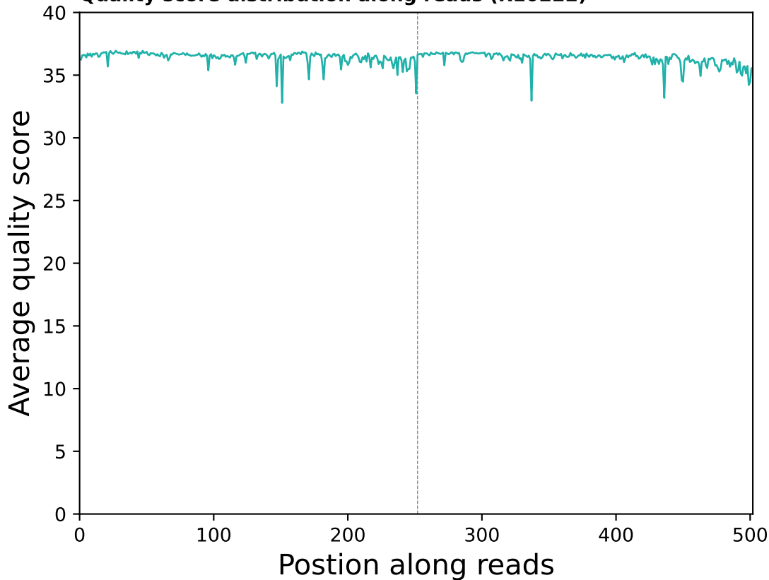
Quality score distribution along reads (R10222)
